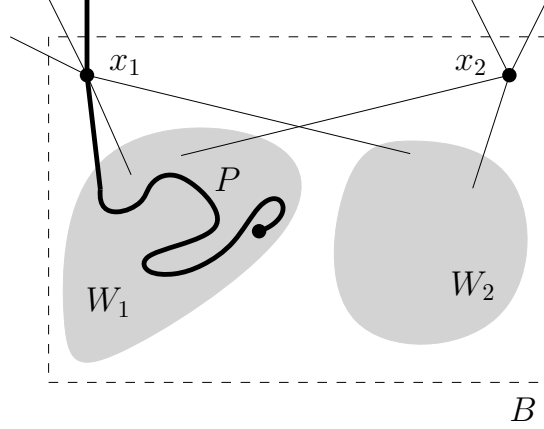
Figure 5: Case k = 2 in the proof of Lemma 16.
