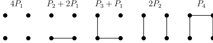
Figure 2: The linear forests on 4 vertices. These are exactly the graphs H on 4 vertices such that \text{Free}(H) is a Gallai family.
