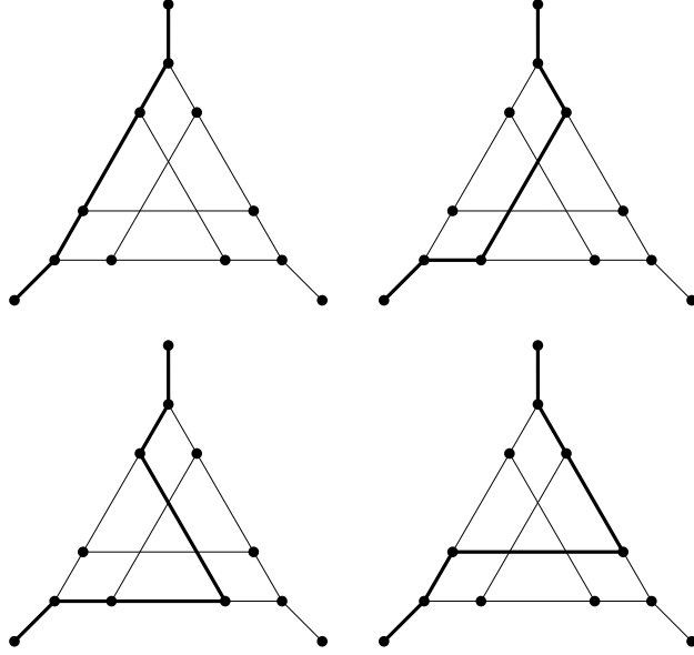
Figure 6: The induced paths in G_0 containing two degree-1 vertices of G_0 .
