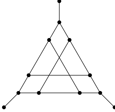
Figure 1: The graph G_0 : A 12-vertex graph with no Gallai vertex.
