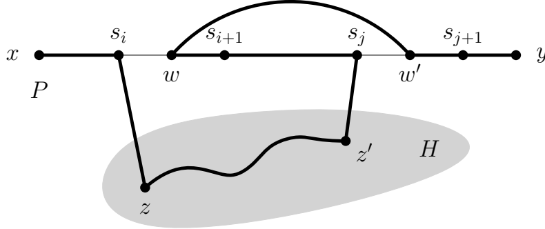
Figure 4: Part 3 in Lemma 8.
